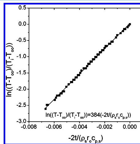
Figure 2. Dimensionless centerline temperature of the copper thermocouple rod (run 2) in the sand bath as a function of modified time. By the assumption of lumped capacitance, the slope of the line is equal to the convection coefficient (eq 20).
