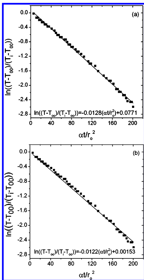
Figure 3. Dimensionless centerline temperature of the copper thermocouple rod (run 2) in the sand bath as a function of dimensionless time. Initial linear fit of eq 25 to the data (a). Linear fit of eq 25 to the data after iteration to reach agreement between eqs 23 and 24 (b).
