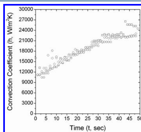
Figure 4. Convection coefficient of steam chamber predicted with eq 6 as a function of time. \square , run 1; \diamond , run 2; \circ , run 3.
