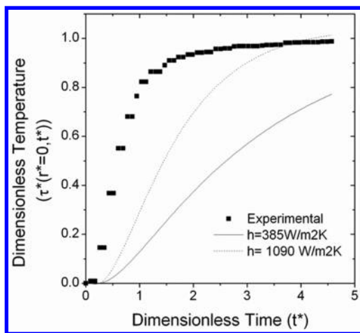
Figure 5. Comparison of dimensionless experimental centerline temperature of the steel thermocouple rod in the steam chamber to those predicted for convection coefficients of 385 \text{W}/(\text{m}^2\cdot\text{K}) (solid line) and 1090 \text{W}/(\text{m}^2\cdot\text{K}) (dotted line) as a function of dimensionless time.
