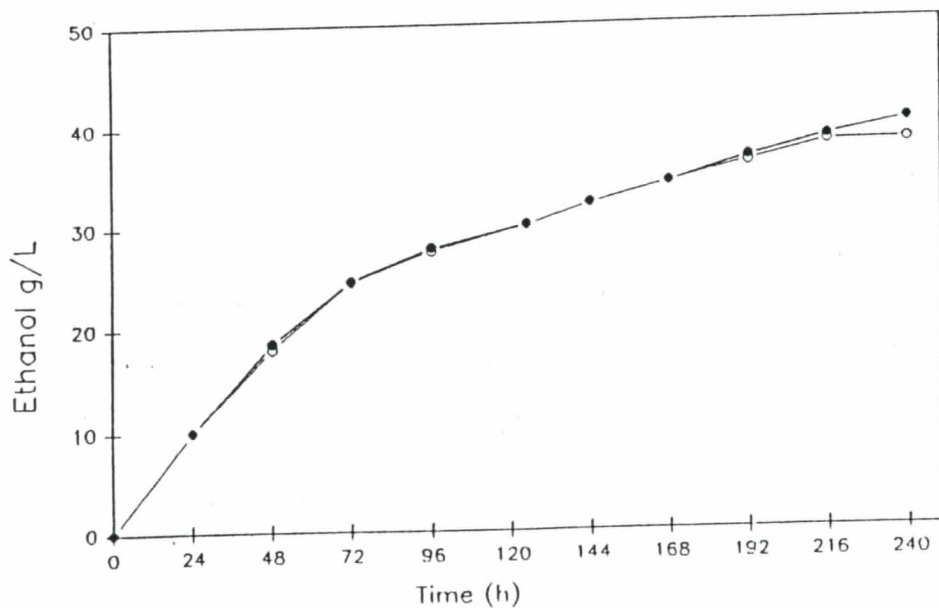
Figure 2. Comparison of ethanol production by B. custersii and a mixed culture of S. cerevisiae and B. clausenii during the SSF of 100 g/L Sigmacell-50 cellulose: (●) B. custersii ; (○) Mixed culture.
