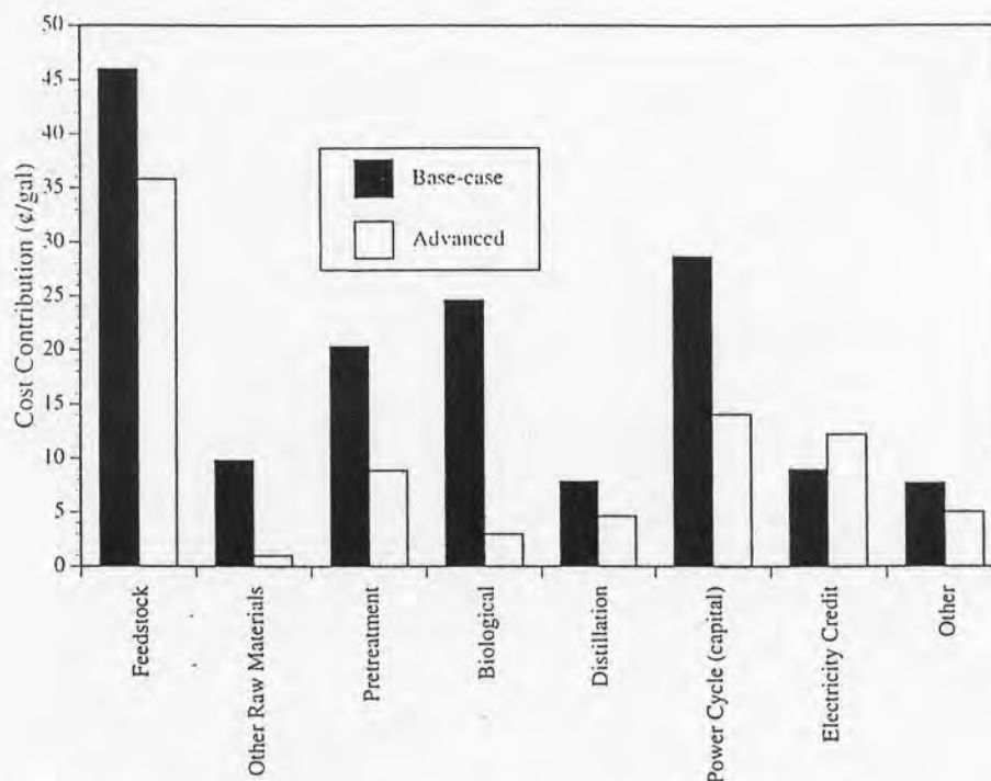
Fig. 1. Comparison of allocated costs for base-case and advanced technology.
